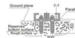
Section of the ground track
