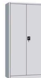
W009 H1850 × W900 × D450mm
