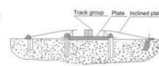
Section of the inclined plate and the surface of the track
