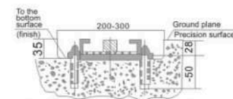
Buried in the ground type track section of the map (reserved groove size)
